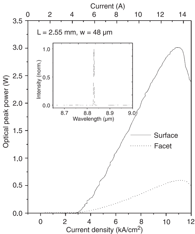
Fig. 2. Absolute light output power versus bias current density for a 2.55 mm long laser at 78 K. The inset shows the spectrum for an applied current of 8 A.
