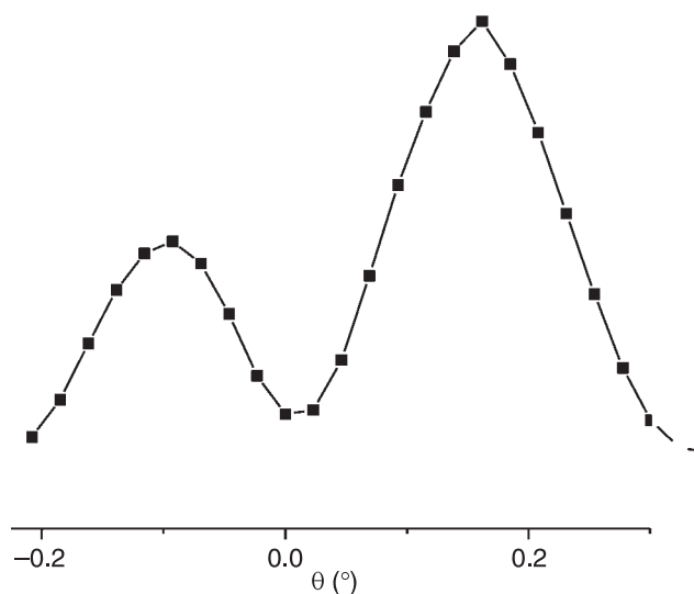
Fig. 3. Far field distribution of the laser emission.
